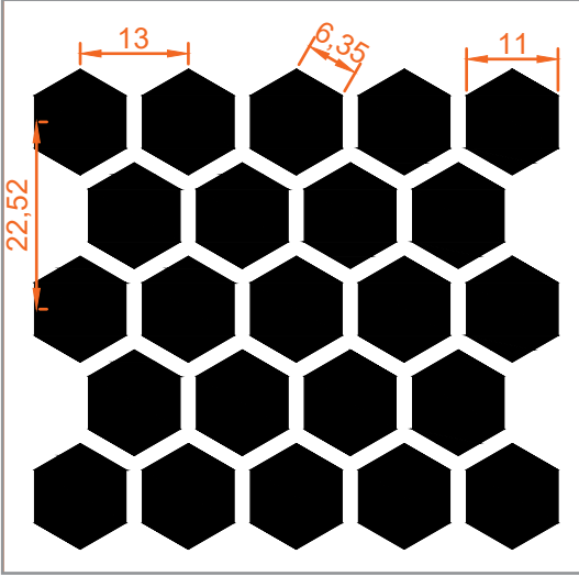
HNY11CNC
